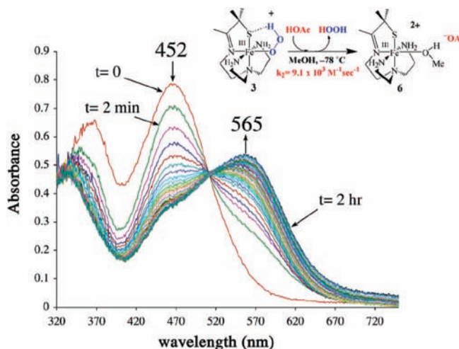
FIGURE 11. Proton-induced conversion of [\text{Fe}^{\text{III}}(\text{S}^{\text{Me}_2}\text{N}_4\text{-tren})(\text{OOH})]^+ ( 3 ) to solvent-bound [\text{Fe}^{\text{III}}(\text{S}^{\text{Me}_2}\text{N}_4\text{-tren})(\text{MeOH})]^{2+} ( 6 ) as monitored by electronic absorption spectroscopy at low temperatures.
