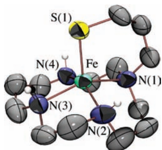
FIGURE 13. ORTEP diagram of trans -thiolate-ligated, biomimetic superoxide reducing catalyst [\text{Fe}^{\text{II}}(\text{cyclam-PrS})]^+ ( 8 ) synthesized by Terutaka Kitagawa, a graduate student in the Kovacs lab.
