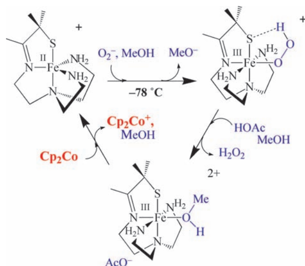
FIGURE 12. Catalytic cycle involving [\text{Fe}^{\text{II}}(\text{S}^{\text{Me}_2}\text{N}_4\text{-tren})]^+ ( 2 )-promoted reduction of superoxide to afford \text{H}_2\text{O}_2 , via the sequential protonation and \text{Cp}_2\text{Co} -promoted reduction of hydroperoxo- and solvent-bound intermediates.
